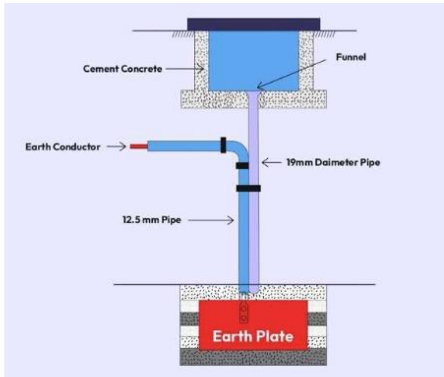
Figure 5.8: Plate Earthing
