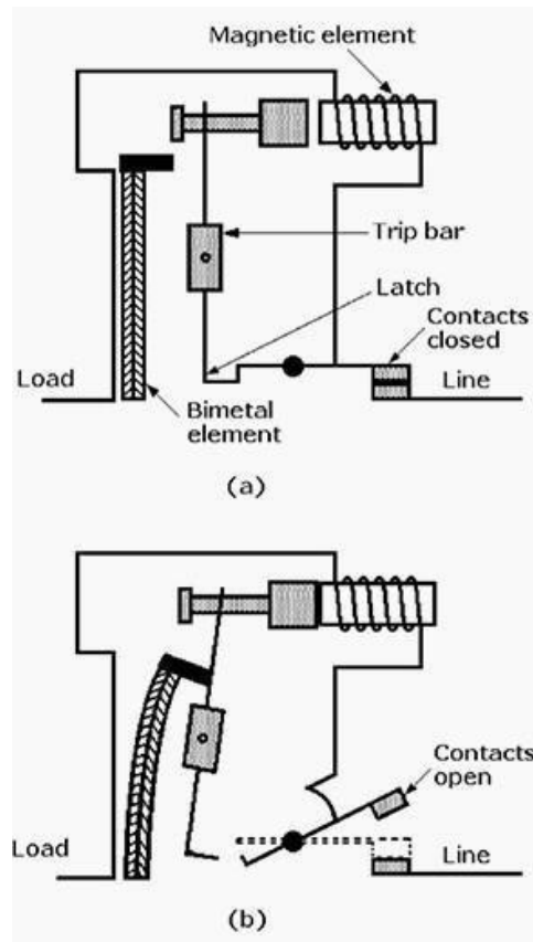
Figure 5.6: MCB Operation
